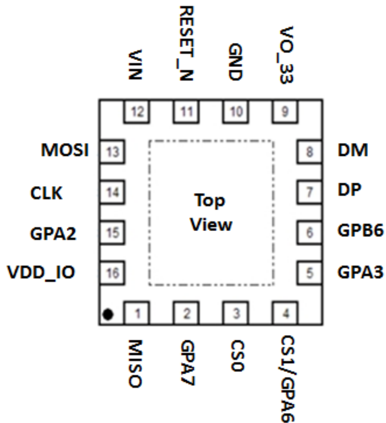
Figure 7-1 PL23D3 Pin Diagram (QFN16)
