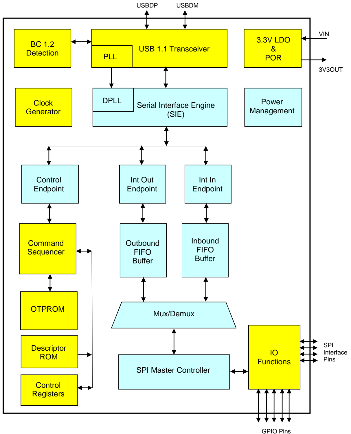
Figure 4-1 PL23D3 Block Diagram
